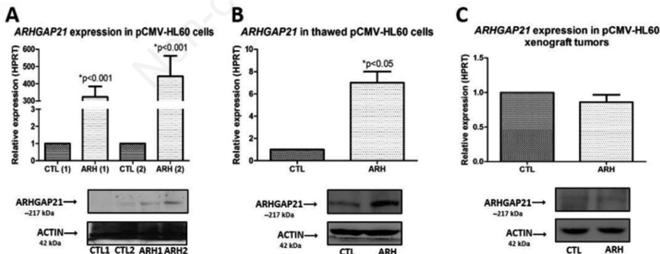
Figure 1. Efficacy of plasmid based gene transfer. (A) Gene (upper panel) and Protein (lower panel) expression of ARHGAP21 in two different pools of HL60 cells transfected with pCMV-ARHGAP21 or pCMV-Control and selected for 10 days with Geneticin; (B) Gene (upper panel) and Protein (lower panel) expression of ARHGAP21 in HL60 cells transfected with pCMV-ARHGAP21 or pCMV-Control after thawing; (C) Gene (upper panel) and Protein (lower panel) expression of ARHGAP21 in xenograft tumors generated by thawed HL60 cells transfected with pCMV-ARHGAP21 or pCMV-Control. HPRT (hypoxanthine phosphoribosyl transferase)=internal control gene for quantitative real-time-PCR expression analysis.
