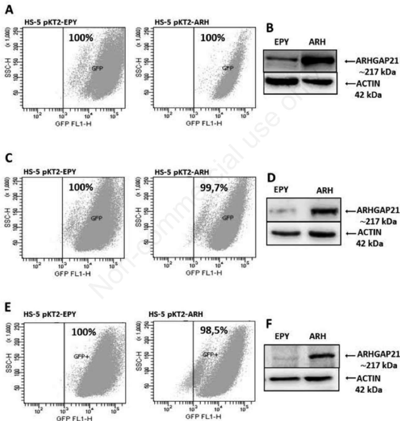
Figure 4. ARHGAP21/iGFP expression in HS-5 cells nucleofected with pKT2-iGFP (pKT2-EPY=empty/control transposon) and pKT2-ARHGAP21-iGFP (pKT2-ARH=ARHGAP21 expression transposon), after 60 days in culture (A and B), after freezing once (C and D) and twice (E and F). The protein expression was verified by Flow Cytometry through GFP tag (A, C and E), and by Western Blotting (B, D and F). ARH=ARHGAP21; EPY=empty; Actin=internal control for protein western blotting expression analysis.
