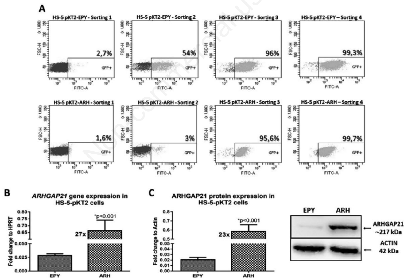
Figure 3. Efficacy of Sleeping Beauty transposon based gene transfer (A) Flow Cytometry showing a gradual increase of GFP + cell populations during purification of HS-5 cells nucleofected with pKT2-iresGFP (pKT2-EPY=empty/control transposon) and pKT2-ARH-iresGFP (pKT2-ARH=ARHGAP21 expression transposon); (B) ARHGAP21 gene expression; (C) ARHGAP21 protein levels in GFP + populations, after purification. ARH=ARHGAP21; EPY=empty; HPRT (hypoxanthine phosphoribosyl transferase)=internal control gene for quantitative real-time-PCR expression analysis; Actin=internal control for protein western blotting expression analysis.
