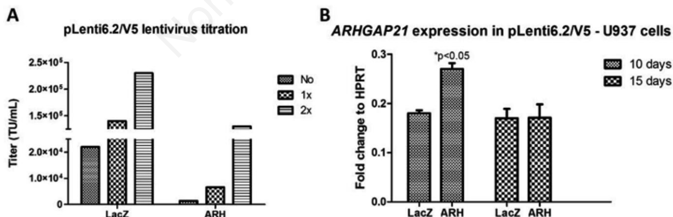
Figure 2. Efficacy of lentiviral based gene transfer. (A) Titration of lentivirus supernatant. The titration was performed in HT1080 cells with supernatant collected from 293FT cells transfected with pLenti6.2/V5-ARH or pLenti6.2/V5-LacZ and submitted to none, one or double ultracentrifugation; (B) ARHGAP21 gene expression in U937 cells transduced with lentivirus supernatant and Blasticidine selected over 10 or 15 days. ARH=sequence which encodes ARHGAP21 protein, co-transfected along with lentivirus packaging vectors to make a recombinant ARHGAP21 lentivirus; LacZ=sequence which encodes the enzyme \beta -galactosidase, co-transfected along with lentivirus packaging vectors to make a recombinant control lentivirus. HPRT (hypoxanthine phosphoribosyl transferase)=internal control gene for quantitative real-time-PCR expression analysis.
