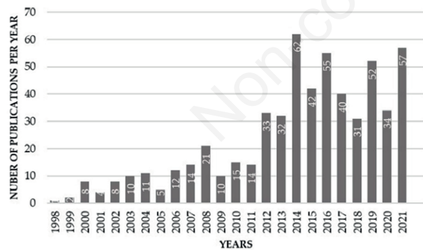
Figure 1. Number of publications indexed in Scopus including the string <<“sea surface salinity” AND (satellite OR “remot* sens*”)>>.
