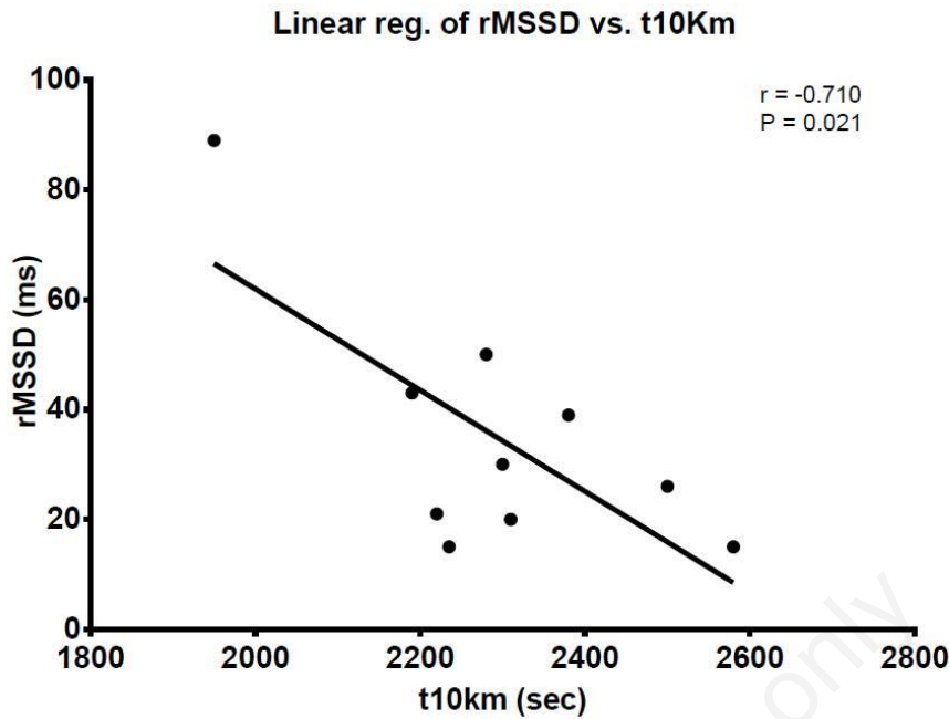
Fig 1. Relationship between time to run 10Km (t10Km) and parasympathetic activity expressed by the square root of the mean squared differences of successive RR intervals (rMSSD)
