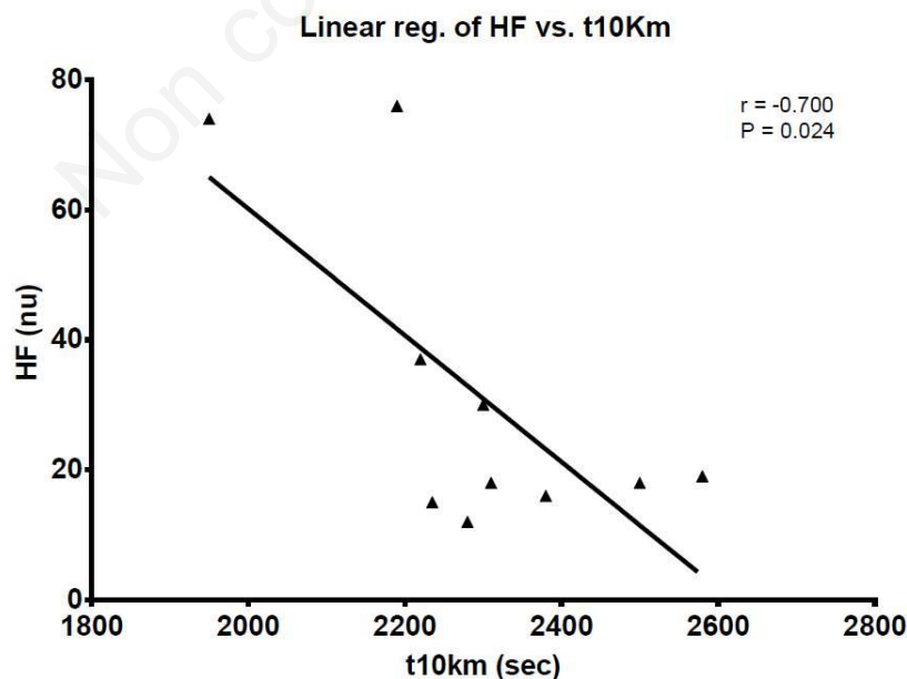
Fig 2. Relationship between time to run (t10Km) and parasympathetic activity expressed by the high frequency power (HF)
