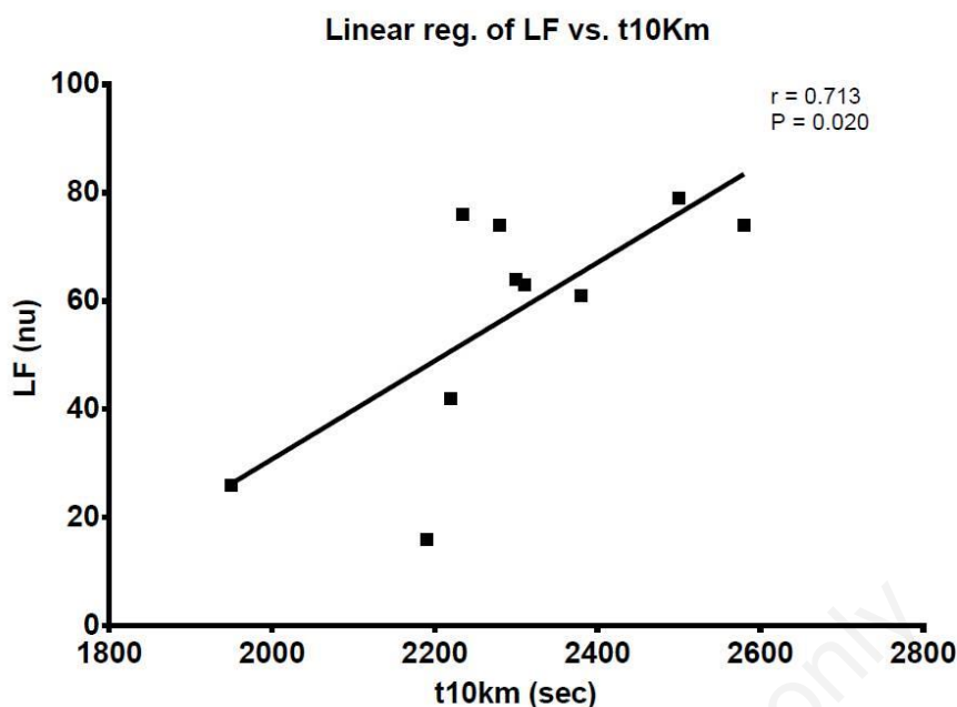
Fig 3. Relationship between time to run (t10Km) and sympathetic activity expressed by the low frequency power (LF)
