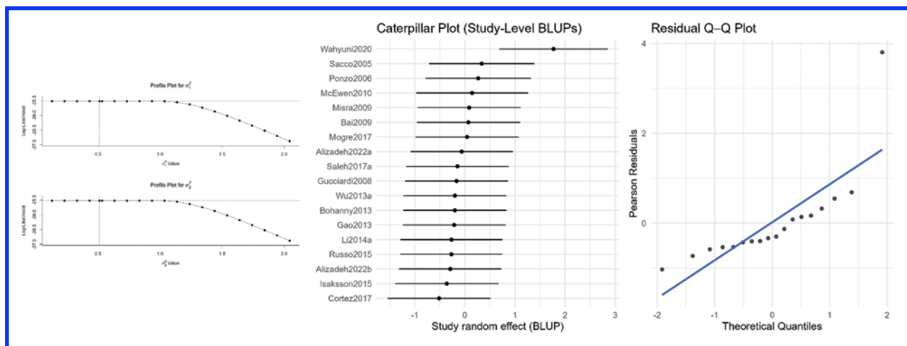
Figure 4. Heterogeneity dashboard: profile-likelihood curves, study BLUPs, and residual Q–Q; Left: profile-likelihood curves for the between- and within-study variance components ( \tau^2 ); curvature indicates identifiable nonzero heterogeneity. Middle: study-level BLUPs with intervals; points near zero indicate small random effects with a few positive deviations. Right: residual Q–Q plot; approximate linearity with an upper-tail deviation suggests a potentially influential positive residual to be examined in leave-one-out diagnostics.
