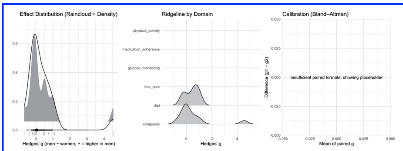
Figure 2. Effect Distribution, Ridgeline by Domain, and Calibration (Bland–Altman); Left: Raincloud and kernel-density plot of Hedges' g (men – women; positive = higher in men) with rug marks for individual study effects. Middle: Ridgeline densities by behavioral domain, illustrating variation across diet, foot-care, glucose-monitoring, medication-adherence, physical-activity, and composite outcomes. Right: Annotated schematic for the Bland–Altman calibration; paired formats were insufficient to permit estimation of cross-format bias, and the panel documents this constraint.
