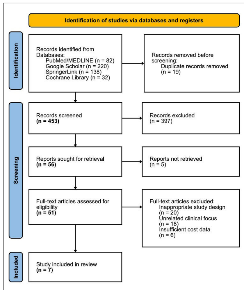
Figure 1. PRISMA flowchart
